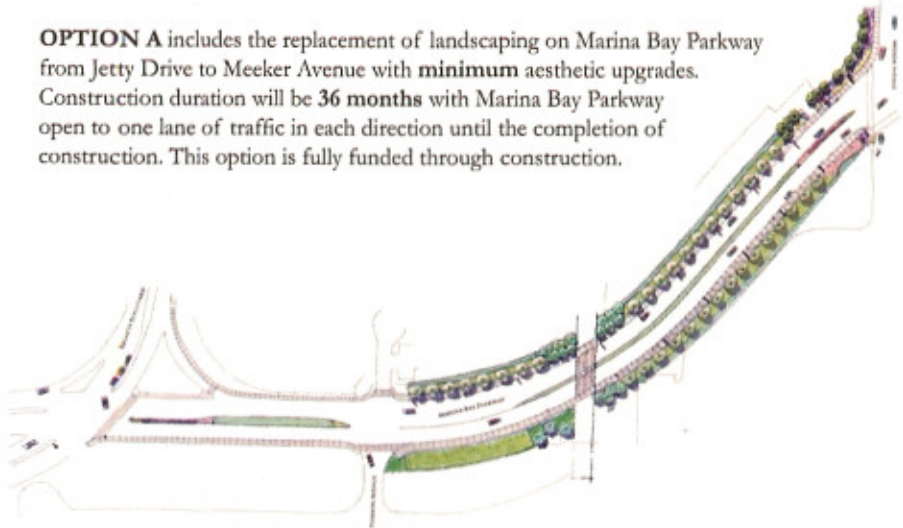
OPTION A: BASE DESIGN PLAN VIEW
